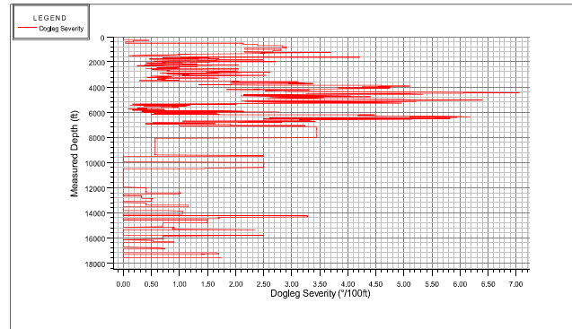
Dogleg Severity
