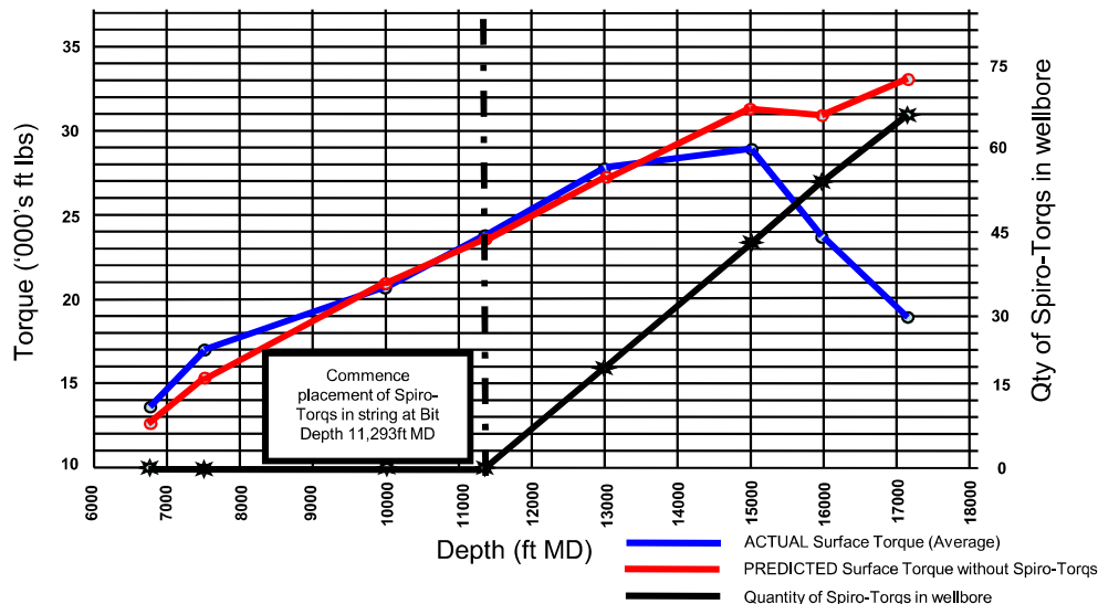
Torque versus Depth
